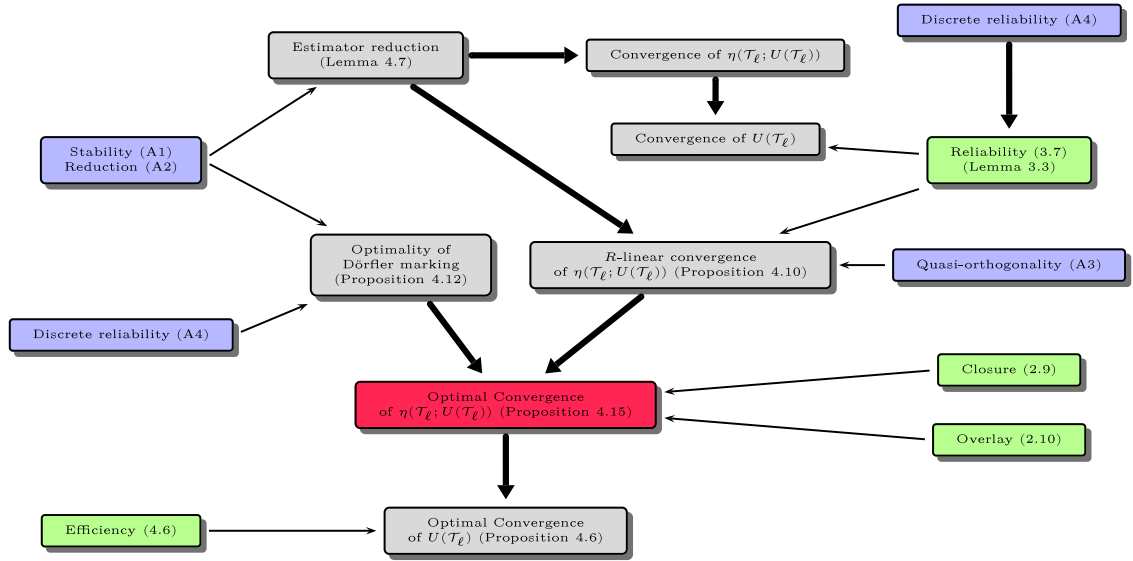
Fig. 1. Map of the quasi-optimality proof. The arrows mark the dependencies of the arguments.
